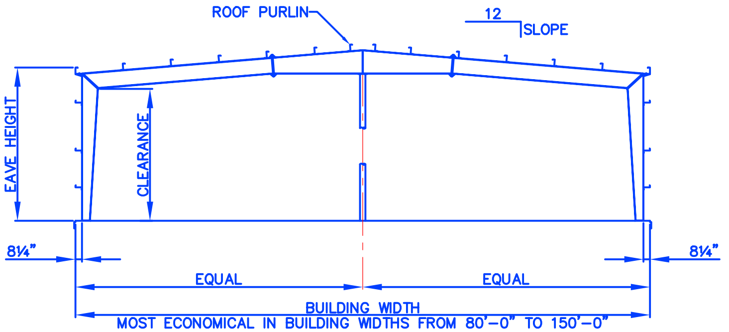
MS1~MODULAR SPAN TAPERED COLUMN BY-PASS GIRT
