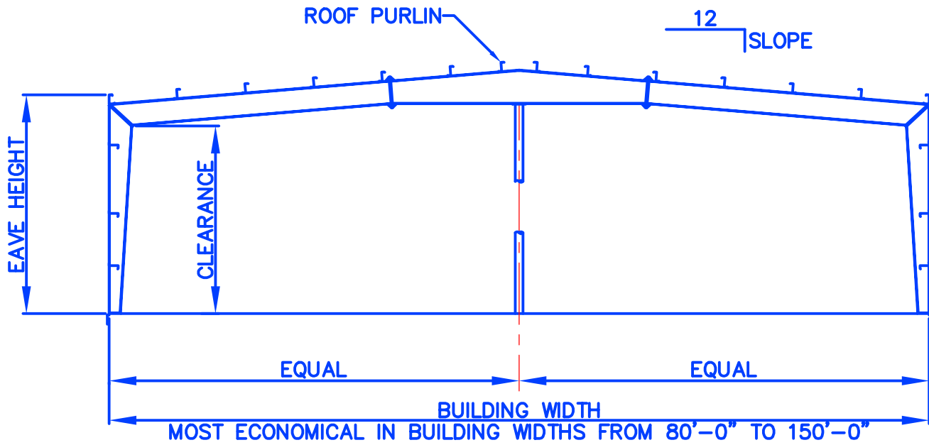
MS1~MODULAR SPAN TAPERED COLUMN FLUSH GIRT
