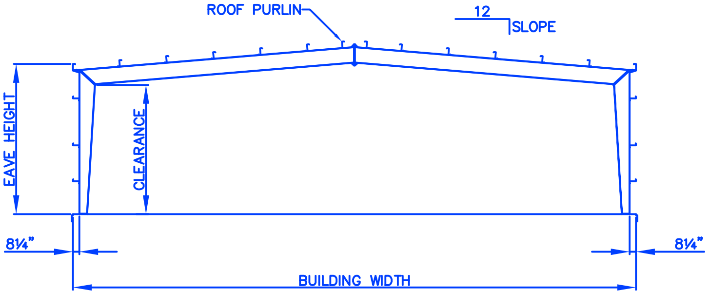
CLEAR SPAN TAPERED COLUMN BY-PASS GIRT
