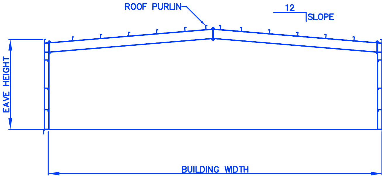
CLEAR SPAN STRAIGHT COLUMN FLUSH GIRT
