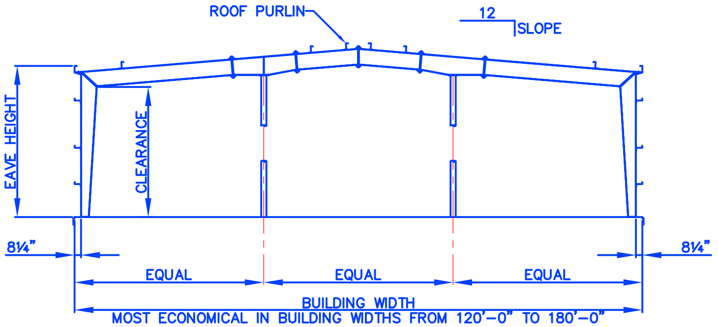
MS2~MODULAR SPAN TAPERED COLUMN BY-PASS GIRT
