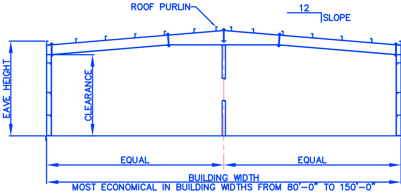
MS1~MODULAR SPAN STRAIGHT COLUMN FLUSH GIRT
