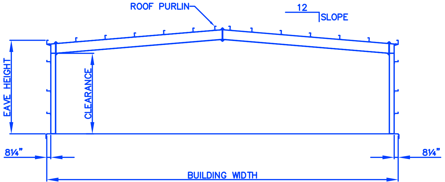
CLEAR SPAN STRAIGHT COLUMN BY-PASS GIRT
