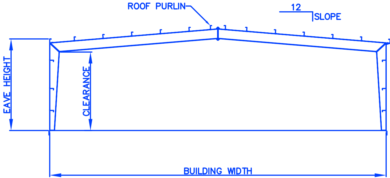
CLEAR SPAN TAPERED COLUMN FLUSH GIRT
