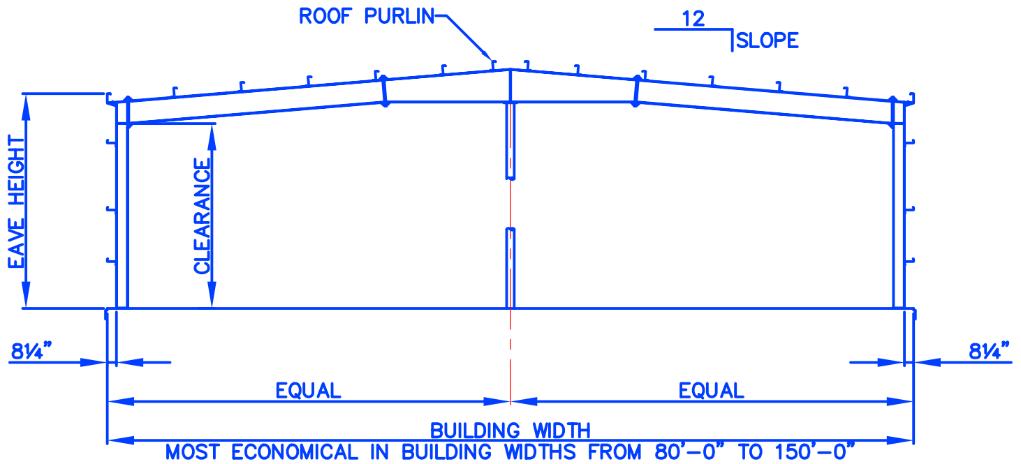
MS1~MODULAR SPAN STRAIGHT COLUMN BY-PASS GIRT
