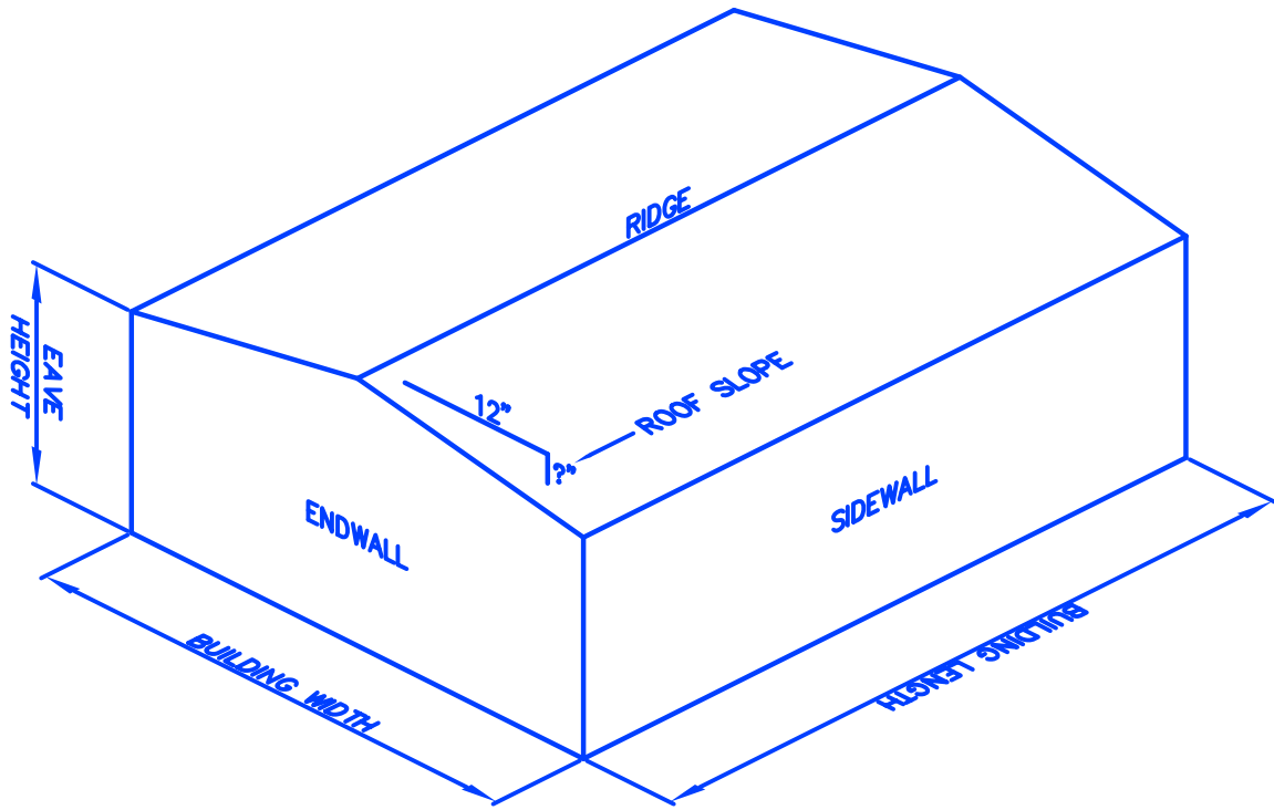
DOUBLE SLOPE BUILDING
